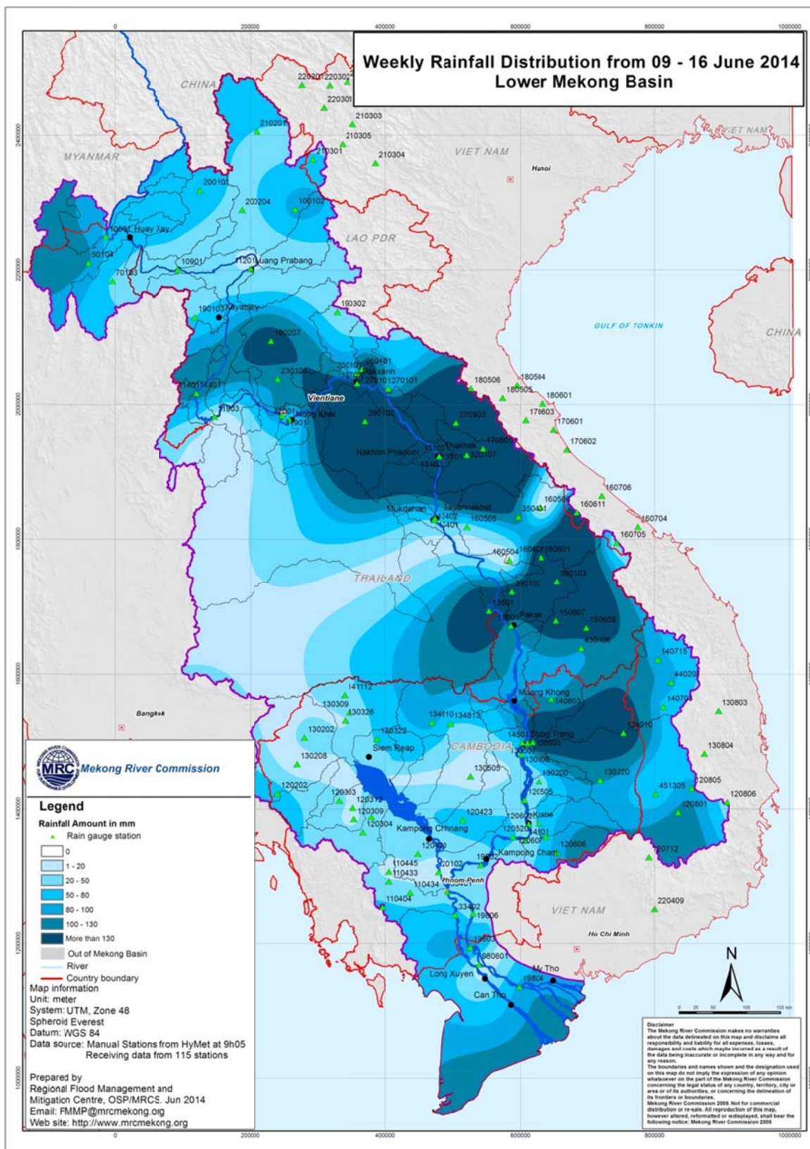
Figure 3: Weekly Rainfall Distribution from 09 th – 16 th June 2014 over the LMB
