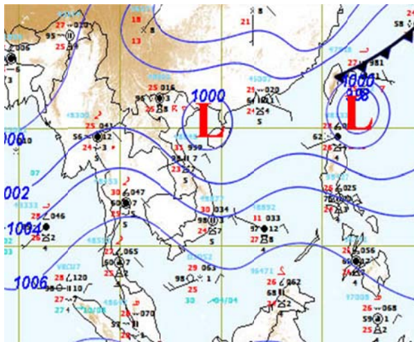
Figure 1: Weather map for 10 th June 2014
