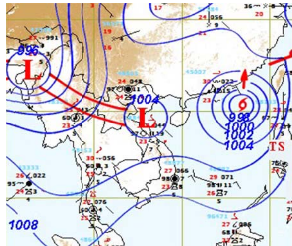
Figure 2: Weather map for 14 th June 2014
